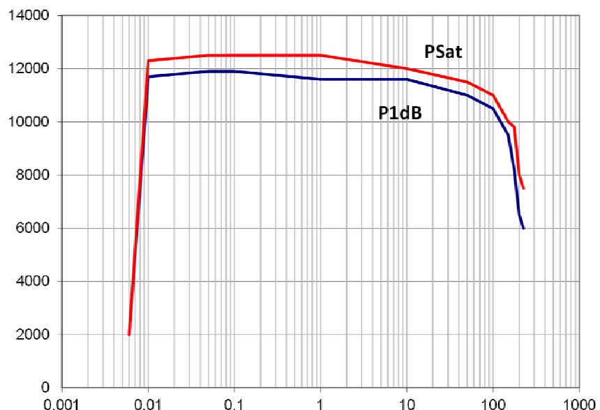
MODEL 12500A225A-L TYPICAL POWER OUTPUT
